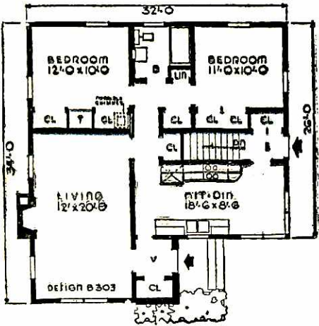
SMALL HOUSE PLANNING BUREAU DESIGN NO. B-303
