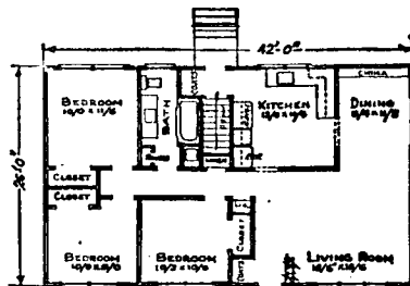
FLOOR PLAN - 1082 Sq. Ft.
