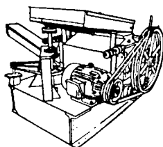
FEED ROLLER MILL
