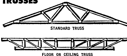
FLOOR OR CEILING TRUSS
